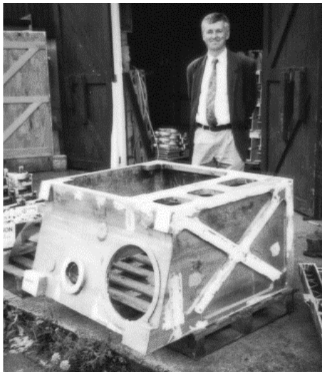
Figure 10. Michelle Vacuum Vessel - Centre Section Casting. Size approx 1.2m square by 0.75m deep.
